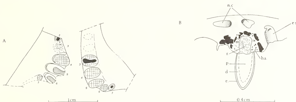
TEXT-FIG. 5. Procolophon trigoniceps . A, palatal view of upper molars of specimen no. B.P.I. 966. Note absence of third right molar and far labial situation of M 7 on both sides. B, Lateral view of lightly ground portion of maxilla of specimen no. B.P.I. 3899. Abbreviations: b.a. bone of attachment; d, dentine; e, enamel; e.s. empty socket; n.c. nutrient canal; p, pulp cavity; r, root.
